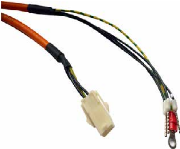
Omron G5 Series 400-750W
