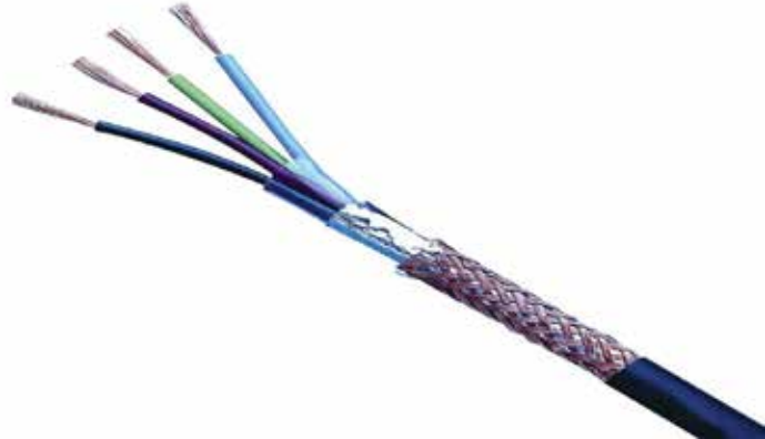
4 CORE * 1.5Sq mm
