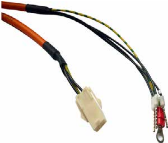
PANASONIC LIQI&A6 POWER CABLE 400-750W
